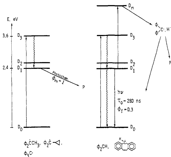
Figure 12. Summary of photophysical and photochemical processes of arylmethyl radicals observed in this study.
