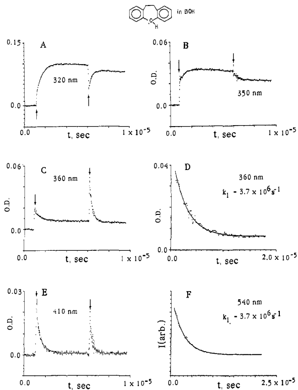
Figure 8. Kinetics of the excited DBHP radicals in EtOH solutions. Radicals were produced by pulse radiolysis of a 2 \times 10^{-3} M solution of the corresponding carbinol: (A–C,E) absorption mode detected at the wavelength indicated; (D,F) least-squares fit (solid curves) to a single exponential decay of the absorption at \lambda = 360 nm (D) and fluorescence at \lambda = 540 nm (F). Note the incomplete recovery of ground state at \lambda = 320 nm and “slow” bleaching at \lambda = 350 nm.
