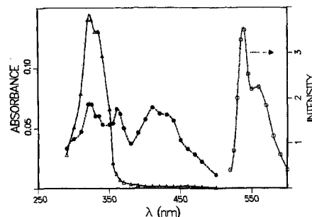
Figure 6. Absorption spectrum of DBHP· radicals in AcN before ( \Delta , solid spectrum) and immediately following the laser flash ( \bullet , dashed spectrum). Dotted spectrum is fluorescence spectrum of the radical; 1 \times 10^{-3} M DBPH-Cl deaerated solution.
