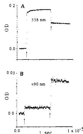
Figure 2. Laser flash photolysis of triphenylmethyl radicals in ethanol. A Ph 3 COH Ar-saturated solution ( 5 \times 10^{-3} M ) in EtOH is used to produce pulse-radiolytically 5 \times 10^{-6} M Ph 3 C \cdot radicals. Linac pulse and laser flash are indicated by the arrows. Wavelengths are indicated.
