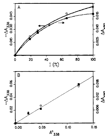
Figure 4. Yield of photolysis products following laser flash photolysis of \text{Ph}_3\text{C}\cdot radicals (A) as a function of laser intensity (40-ns linac pulse) and (B) as a function of linac dose (represented as absorbance of radiolytically produced radicals): (O) measured as bleaching at \lambda = 338 nm, (●) measured from absorption of products at \lambda = 480 nm; 10^{-3} \text{ M} \text{Ph}_3\text{CCl} in AcN.
