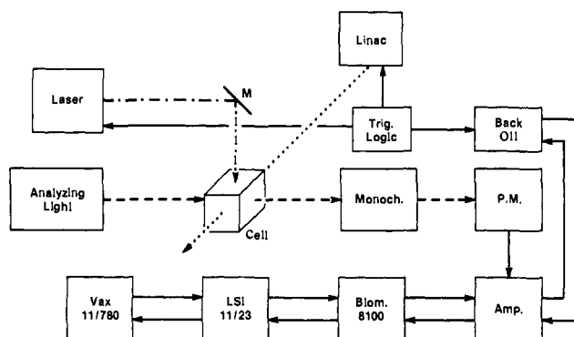
Figure 1. Schematic presentation of the pulse radiolysis/laser flash photolysis system.
