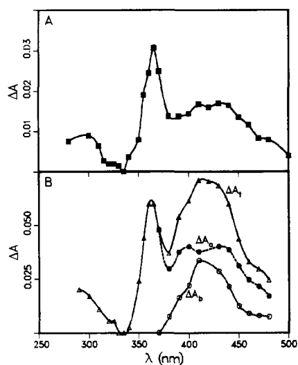
Figure 10. Absorption spectra of the first excited state of DBHP• radicals in CHX (A) and in AcN (B) with its photolysis products. \Delta A_t is the total absorbance change (corrected for ground-state bleaching) immediately following the laser flash; \Delta A_a is the absorbance due to the fast exponential decay, and \Delta A_b is the fraction due to the slow decay. At \lambda < 370 nm only one process is observed. Experimental conditions as in Figure 8.
