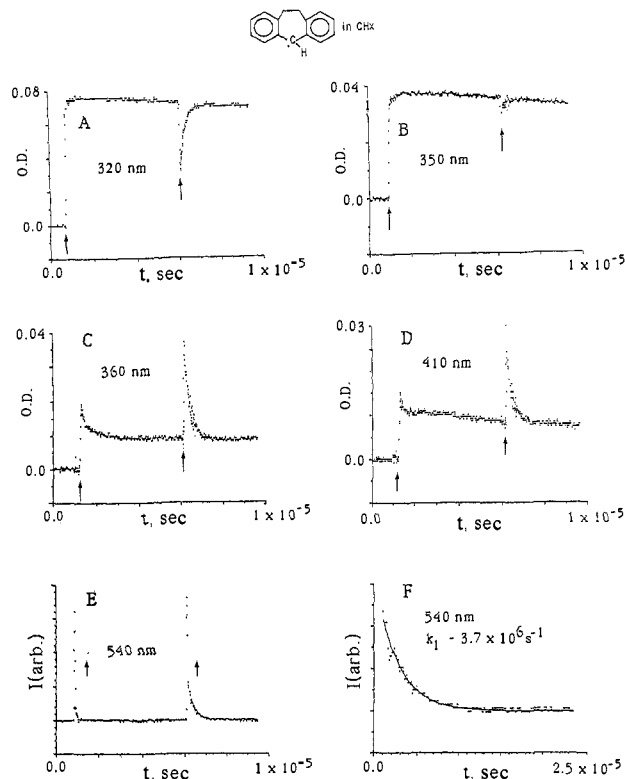
Figure 7. Kinetics of excited DBHP· radicals, produced by pulse radiolysis of a 2 \times 10^{-3} M solution of the corresponding carbinol in CHX: (A) \lambda = 320 nm, bleaching of the ground state; (B) \lambda = 350 nm, nearly isosbestic point of the ground and excited states; (C,D) \lambda = 360, 410 nm, absorption maxima of the first excited doublet; (E) fluorescence at \lambda = 540 nm; and (F) least-squares fit (solid curve) to a single exponential decay of the fluorescence at \lambda = 540 nm.
