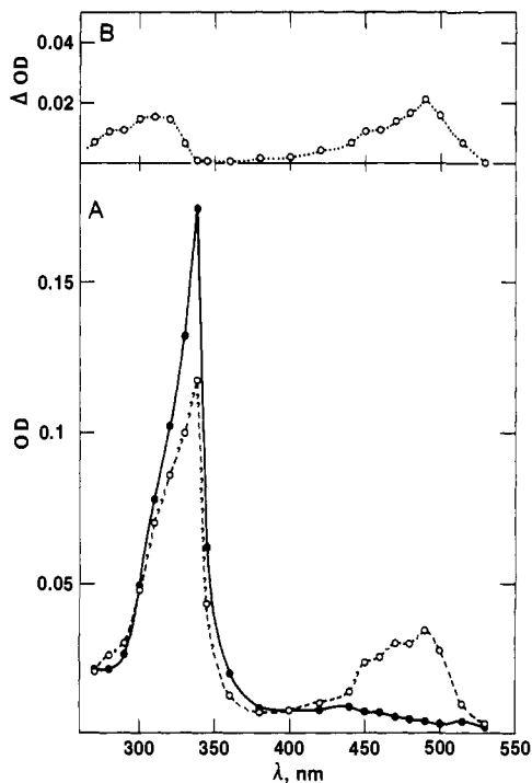
Figure 3. (A) Absorption spectrum of \text{Ph}_3\text{C}\cdot radicals in EtOH before (solid line) and after (dashed spectrum) the laser flash. (B) Absorption spectrum of the photolysis product of \text{Ph}_3\text{C}\cdot calculated assuming no absorption of the products at the absorption maximum (338 nm) of the radical (see text). Experimental conditions as in Figure 2.
