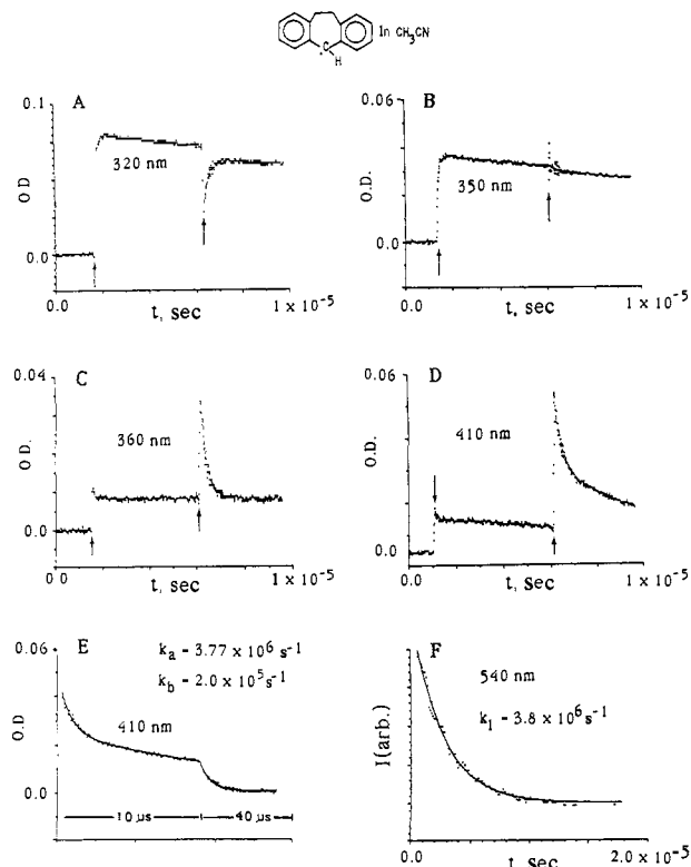
Figure 9. Photochemistry of DBHP• radicals in AcN. Experimental conditions as in Figure 8: (A–D) absorption signals at the indicated wavelengths; (E) least-squares fit of the decay of the absorption at \lambda = 410 nm assuming two exponential decays, one of which fixed at k_a = 3.77 \times 10^6 \text{ s}^{-1} (solid curve); (F) monoexponential decay of fluorescence at \lambda = 540 nm.
