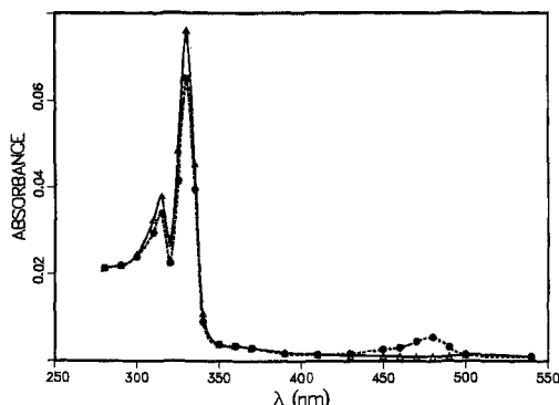
Figure 5. Absorption spectrum of pulse-radiolytically produced \text{Ph}_2\dot{\text{C}}\text{CH}_3 radicals before ( \Delta , solid spectrum) and immediately following ( \bullet , dashed spectrum) the laser flash: 10^{-2} M \text{Ph}_2\text{C}(\text{CH}_3)\text{OH} in Ar-saturated AcN solution.
