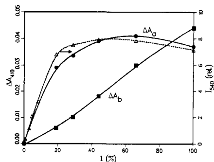
Figure 11. Effect of laser light intensity on fluorescence intensity ( I_{540} ) and on absorbance of the lowest excited state ( \Delta A_a , measured at 410 nm) and of the photochemical product ( \Delta A_b , measured at 410 nm) for DBHP• radicals in AcN. Experimental conditions as in Figure 8.
